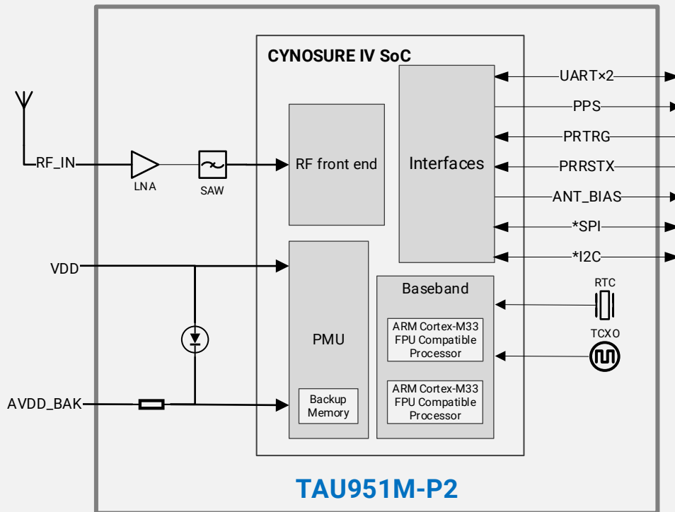
Figure 2 Block diagram
