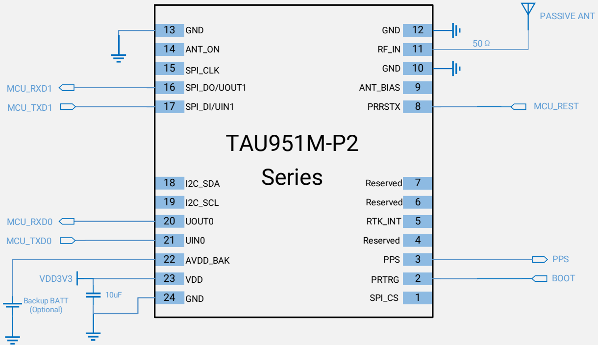
Figure 10 Reference design of passive ant.
