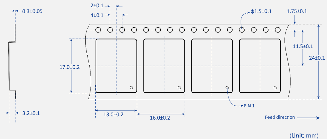
Figure 12 Tape dimensions
