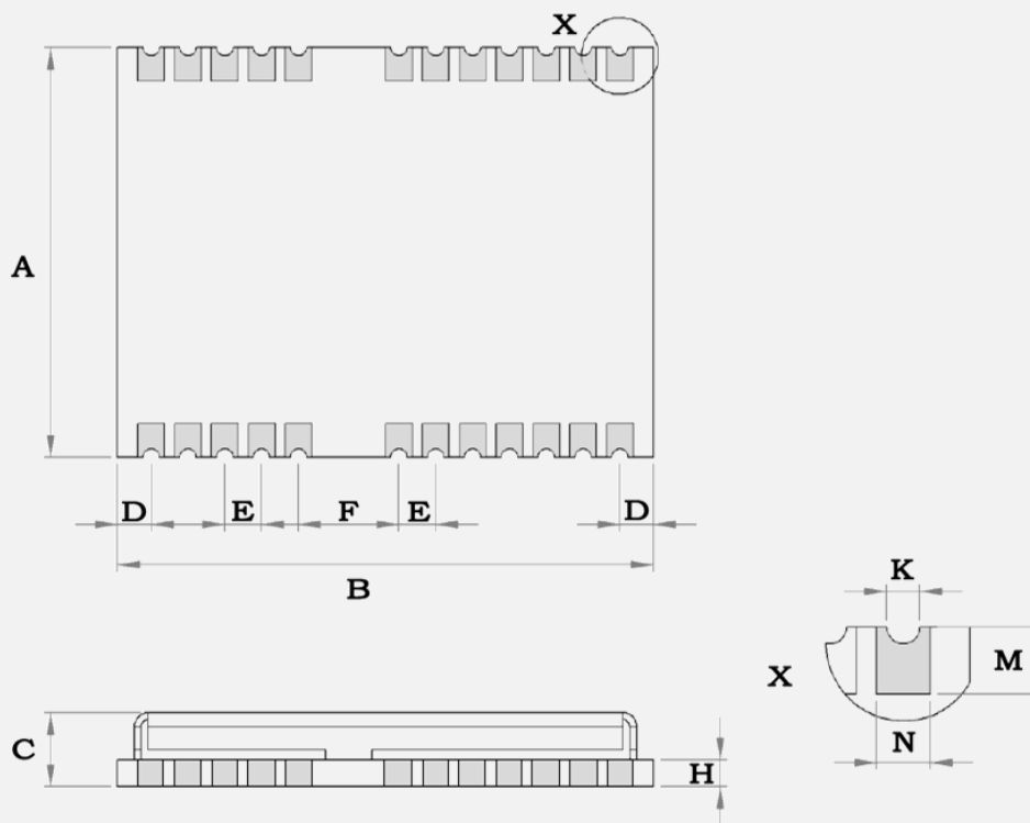
Figure 7 Dimensions
